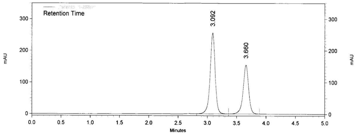
Figure 31: Chromatogram of reference formulation
